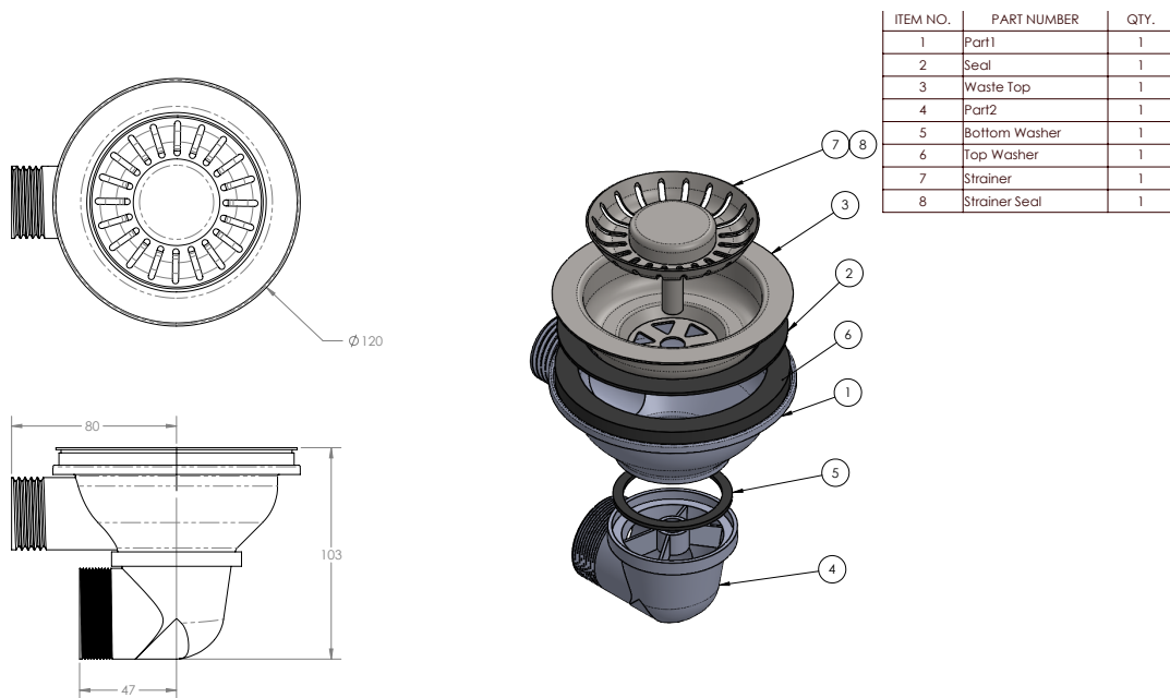
Part No. 7 Replacement basket waste - WBP175704 · AW704 Designer Basket Waste Replacement
