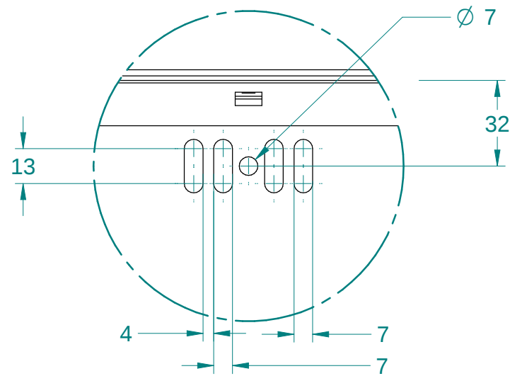
DETAIL A 1:2
