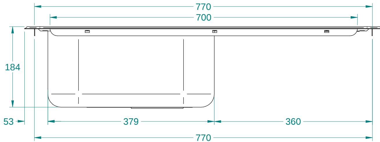
DETAIL A 1:2
