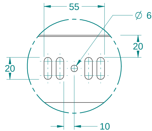
DETAIL A 1:2
