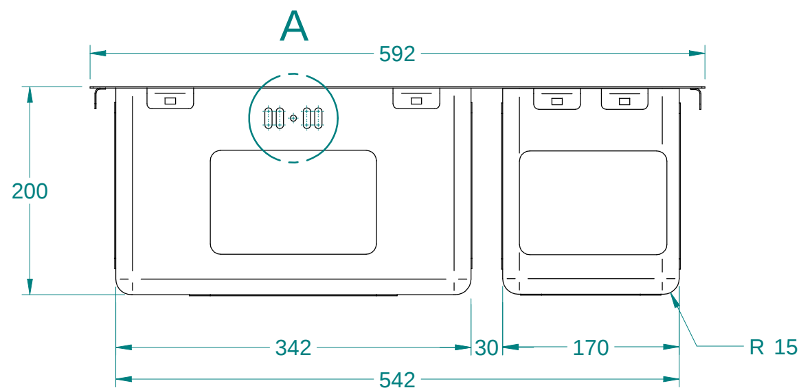
DETAIL A 1:2
