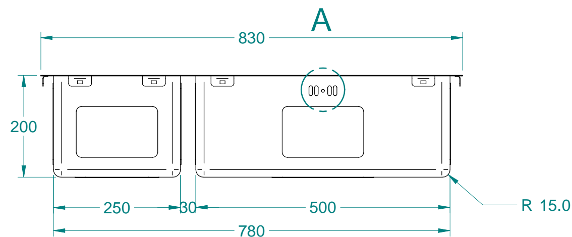
DETAIL A 1:2
