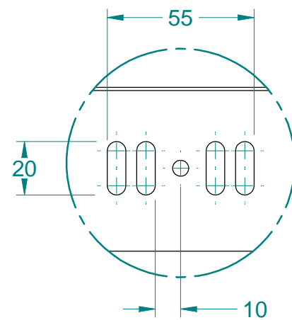
DETAIL A 1:2
