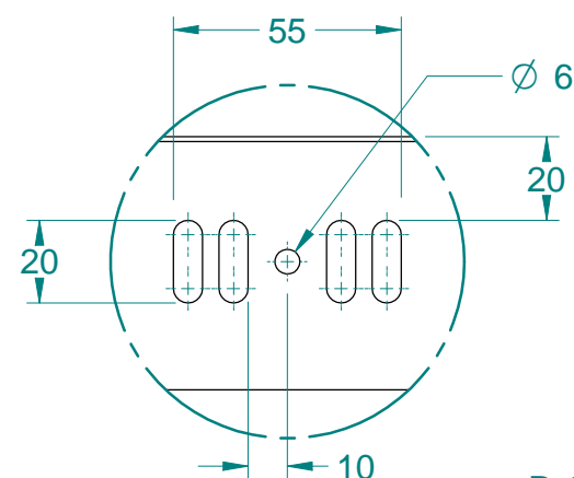
DETAIL A 1:2
