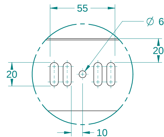
DETAIL A 1:2
