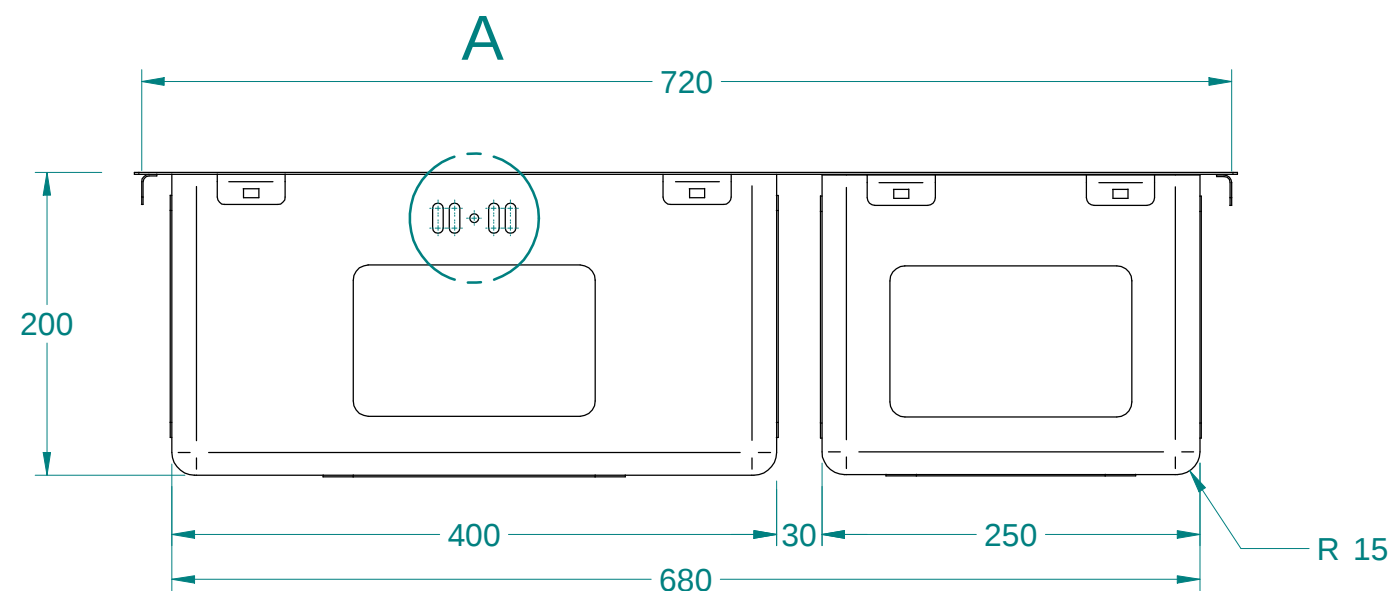
DETAIL A 1:2
