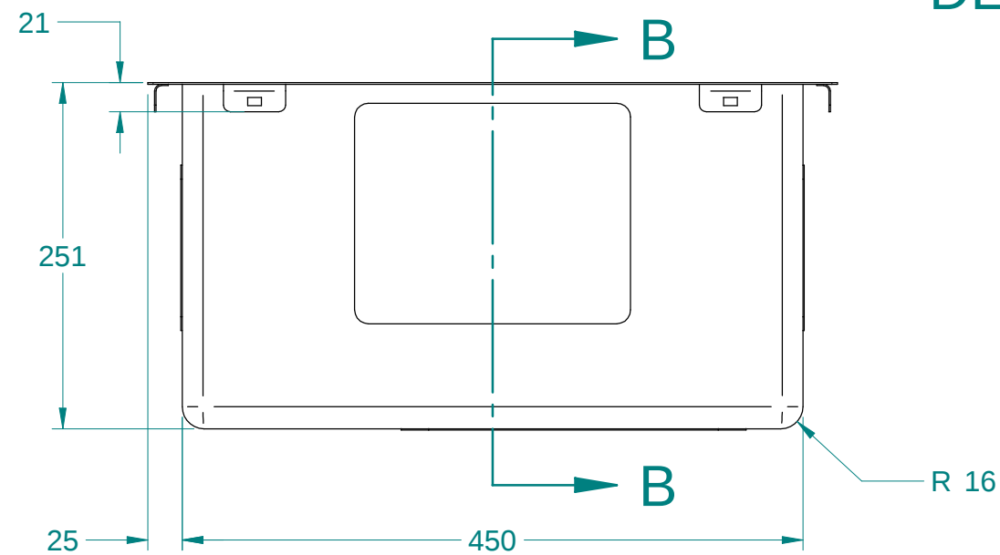
DETAIL A
