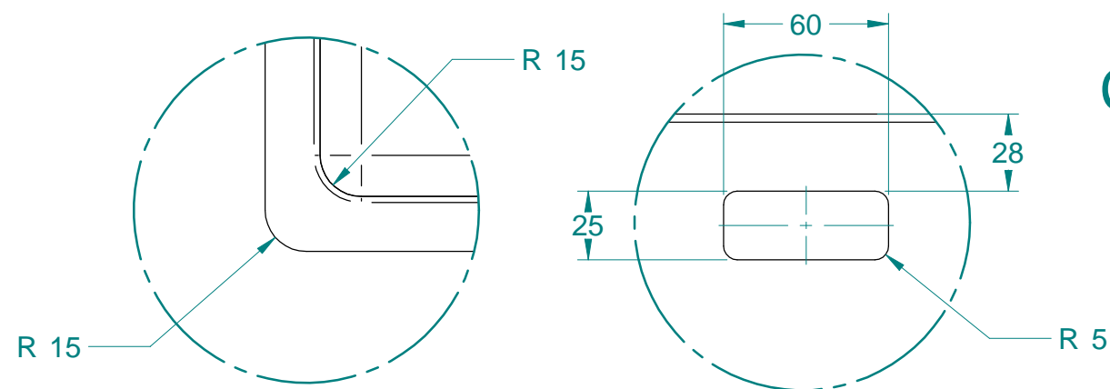
DETAIL C 1:2.5
