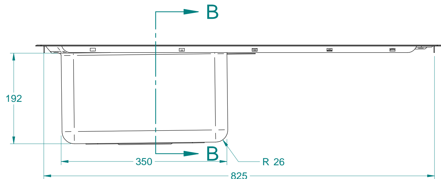
DETAIL A
