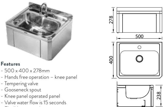
HFB3 Hand Wash Basin Knee Operated
