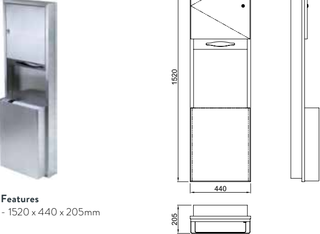
PTC1 Paper Towel Cabinet
