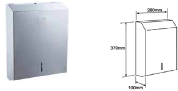
PTD1 Paper Towel Roll Dispenser
