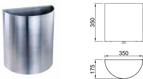
RB1 Rubbish Bin
