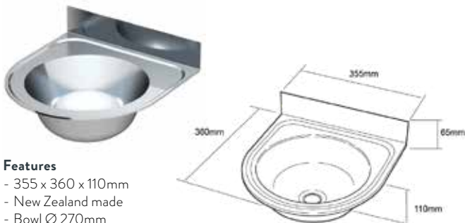
G7 Hand Wash Basin Round Bowl Round
