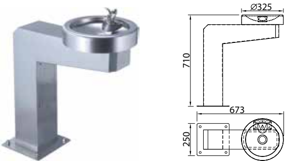
DF5 Drinking Fountain Floor Standing Disabled
