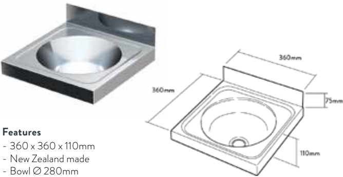
G4 Hand Wash Basin Round Bowl Square
