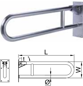
GRMH2 Grab Rail Movable Hinge
