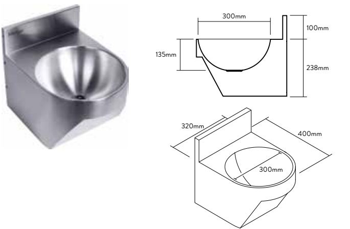
HWB6 Accessible Hand Wash Basin Round Bowl
