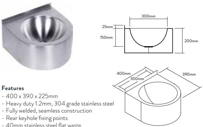
HWB4 Hand Wash Basin Round Bowl
