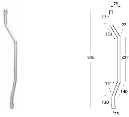
DP2 Drop Pipe Single Urinal
