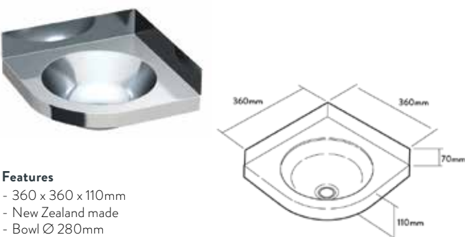
G6 Hand Wash Basin Round Bowl Corner
