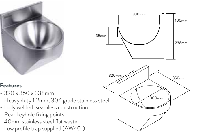
HWB5 Hand Wash Basin Round Bowl Compact
